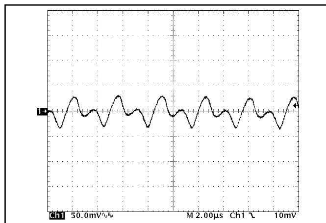
Figure 16: Output voltage ripple at nominal input voltage and rated load current (50 mV/div). Load capacitance: 1\ \mu\text{F} ceramic capacitor and 15\ \mu\text{F} tantalum capacitor. Bandwidth: 20 MHz. See Figure 13.
